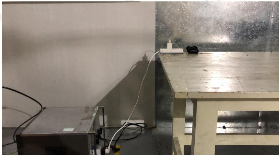
Conducted Emission
