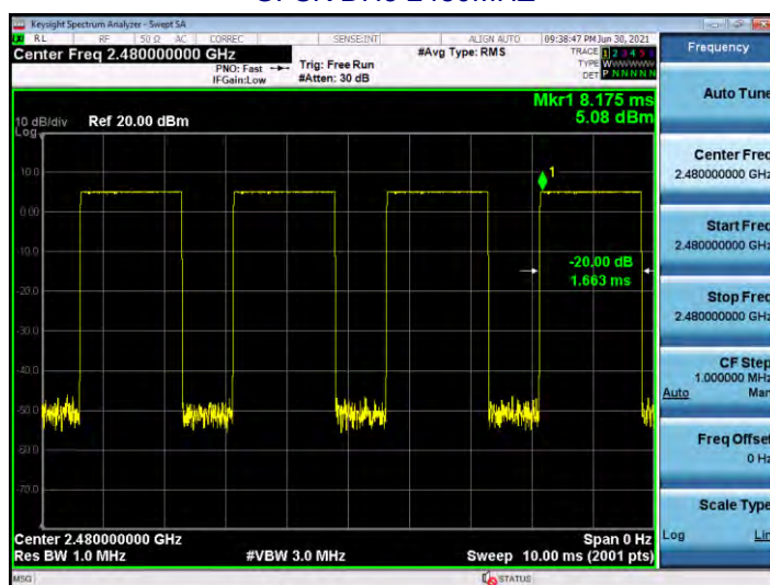
GFSK DH3 2480MHZ
