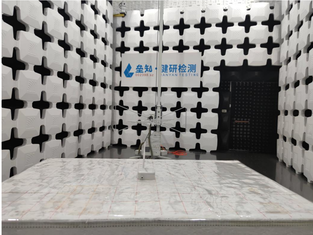
Radiated Spurious Emission External antenna Below 1GHz
