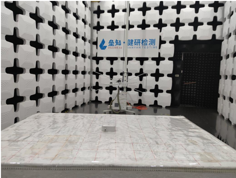
Radiated Spurious Emission Internal antenna Below 1GHz
