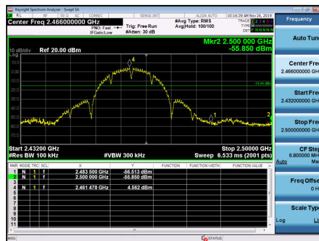
Right bandedge
