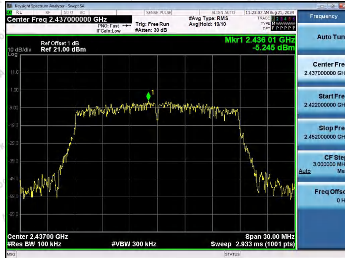
11N20SISO-Ant1-2437-0~Reference-PASS
