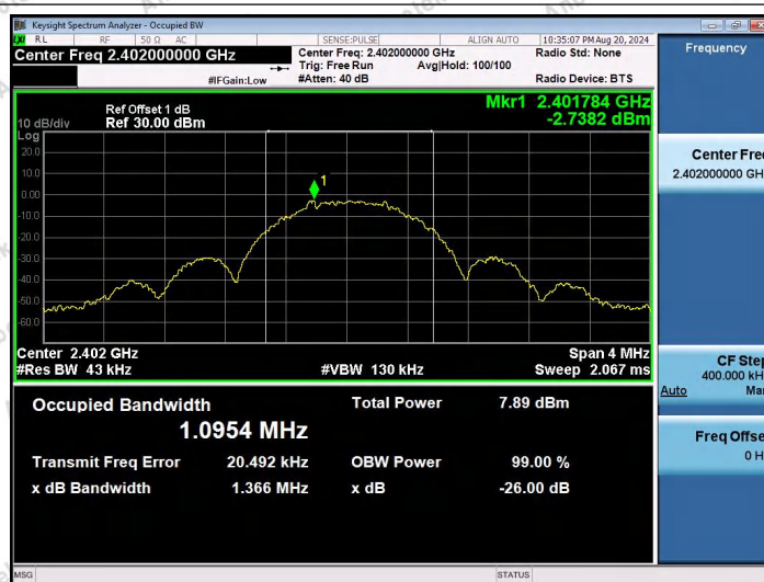
BLE_1M-Ant1-2402
