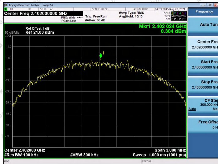
BLE_2M-Ant1-2402-0~Reference-PASS
