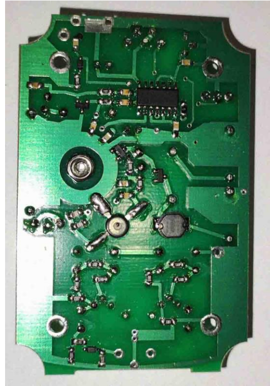
Zond Aero 500 Transmitter top and bottom view
