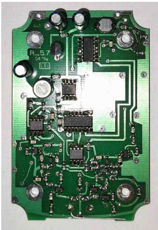
Zond Aero 500 Receiver top and bottom view
