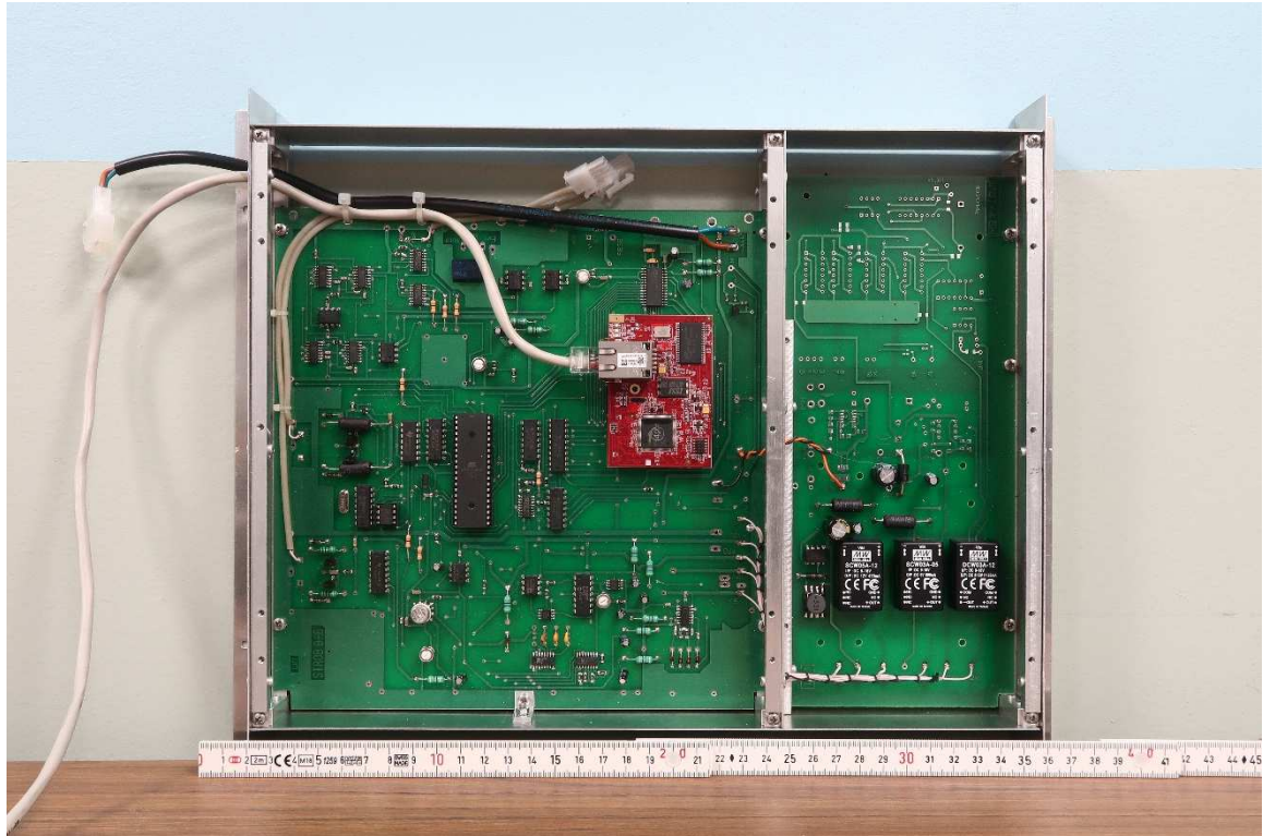
Chassis Top (Cover removed)
