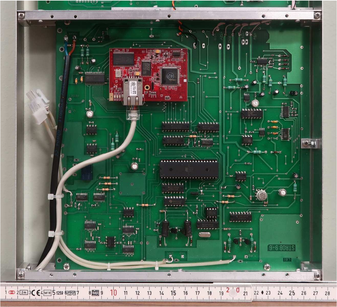
Control Unit Large Module – Front
