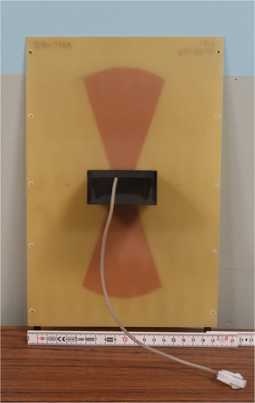
Tx Antenna Back
