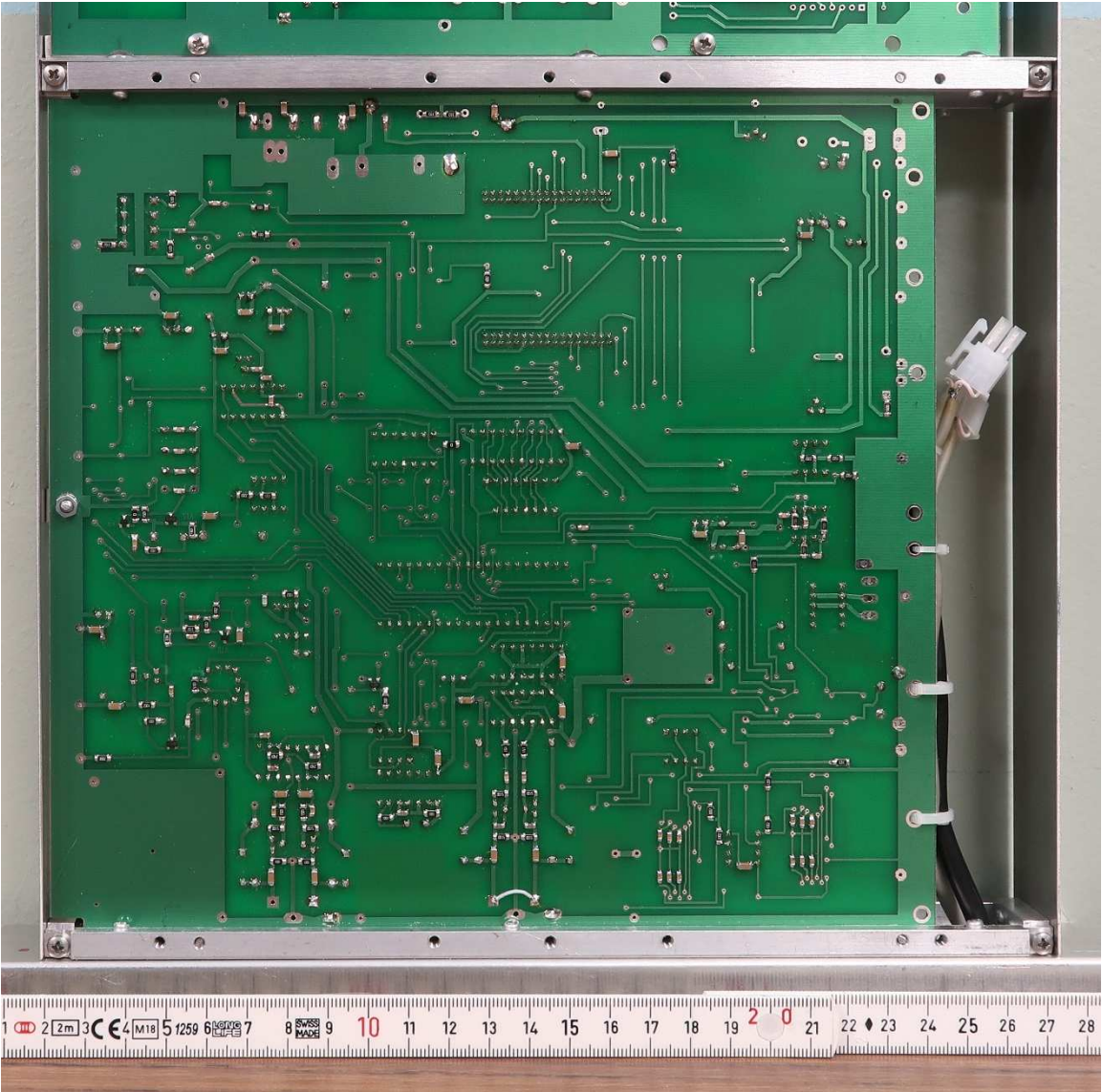
Control Unit Large Module – Rear
