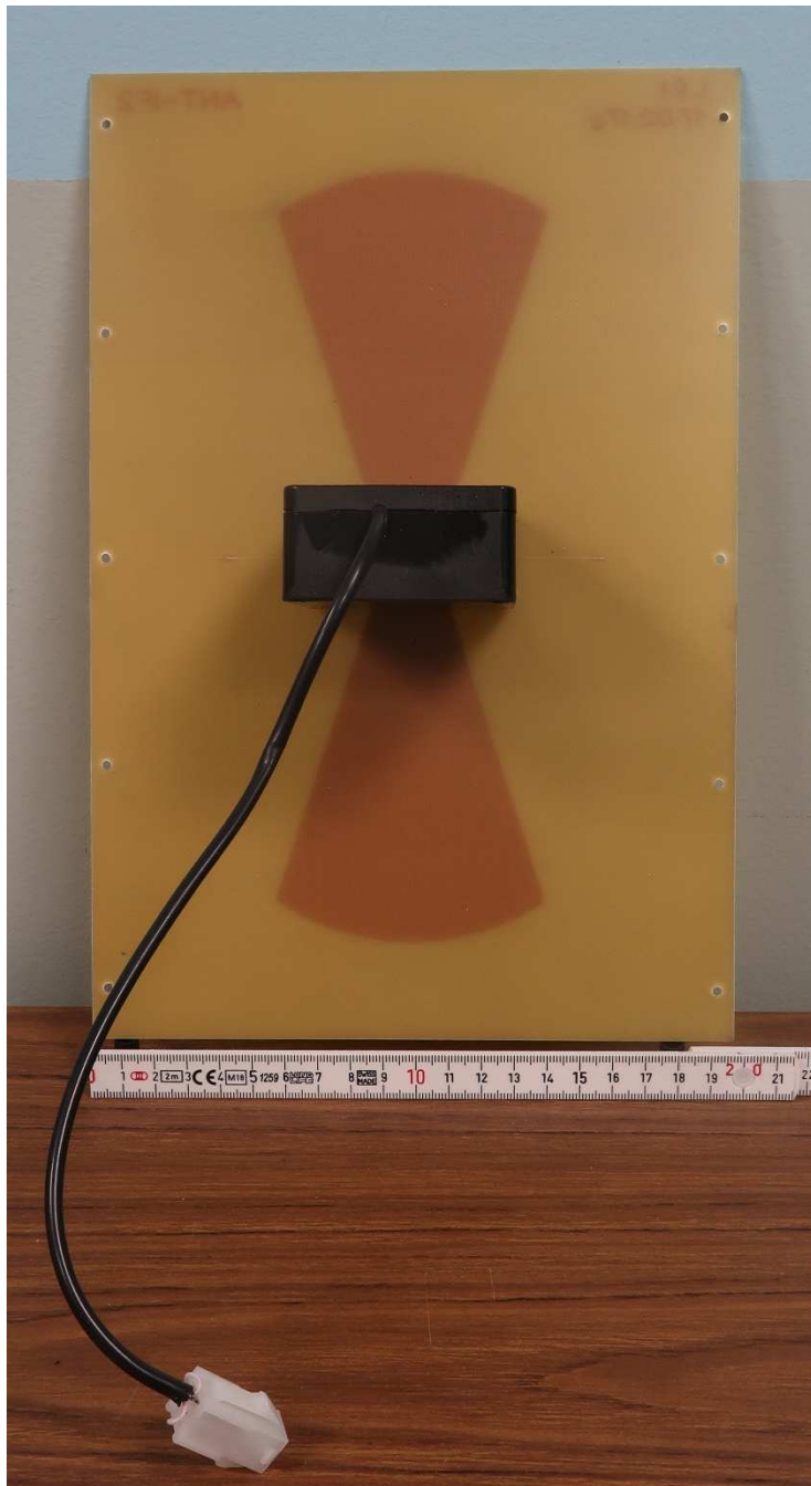
Rx Antenna Back
