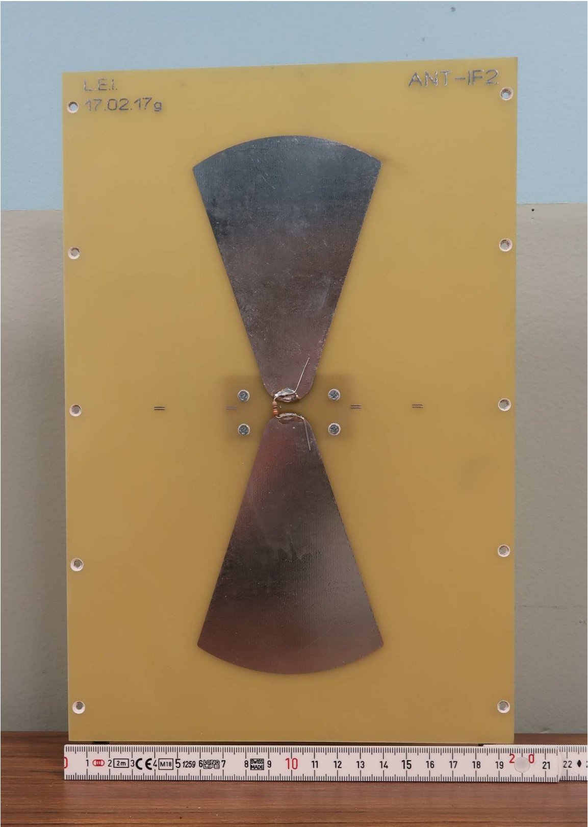
Tx Antenna Front
