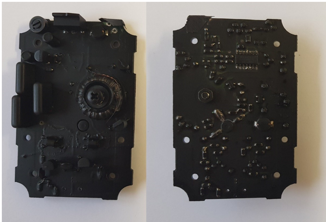
Zond-12e 500A Transmitter top and bottom view with moisture protection
