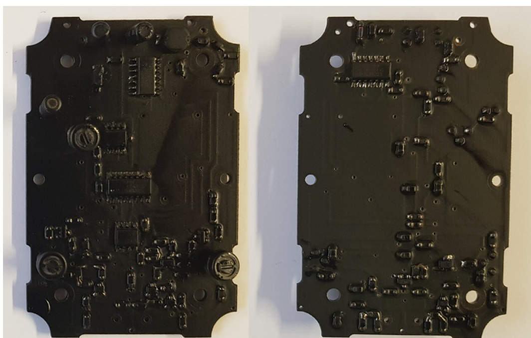
Zond-12e 500A Receiver top and bottom view with moisture protection
