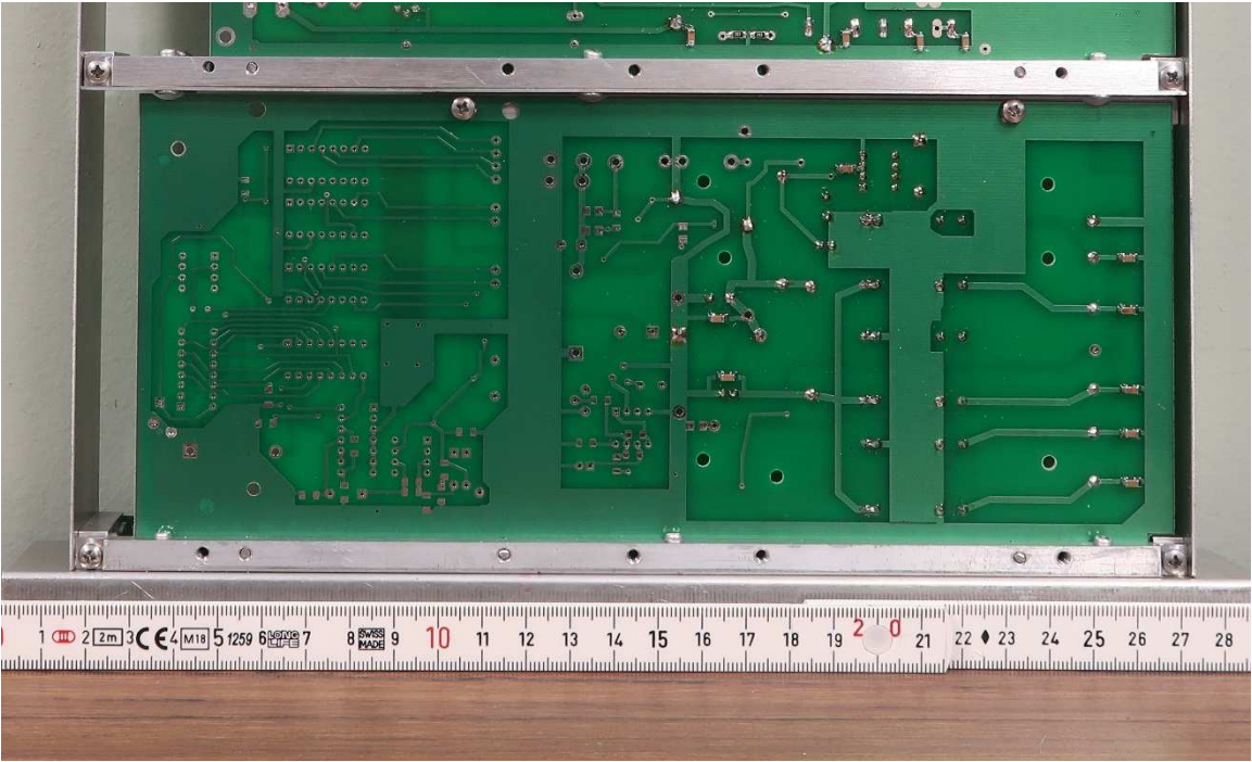
Control Unit Small Module – Rear
