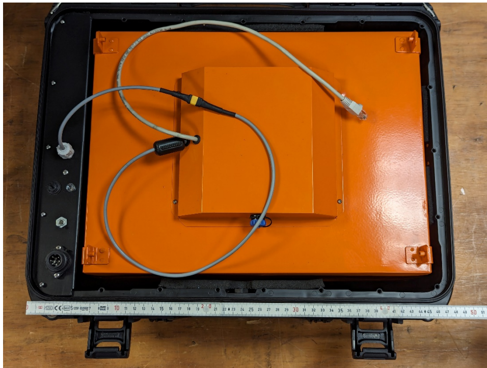
Top with Cover Open
