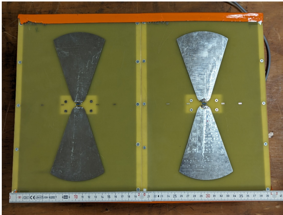
Bottom View Removed from Case
