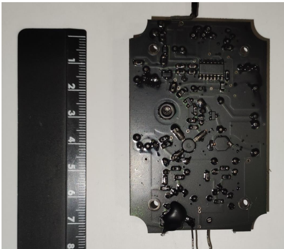
Zond Aero 500 NG Transmitter top and bottom view
