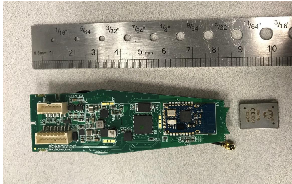
PCB Bottom View with BLE Shield removed
