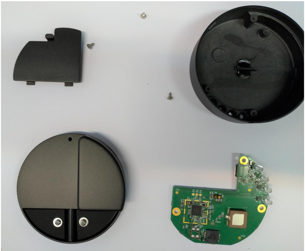
Picture 2. Jiffy Dongle - Desktop Version - all parts separated
