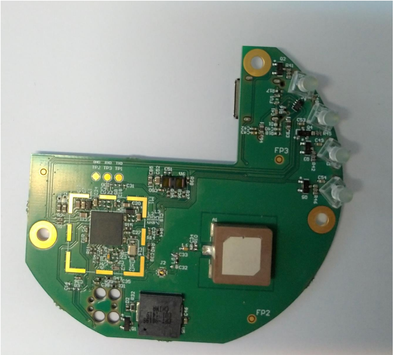
Picture 4. Jiffy Dongle - Desktop Version - PCB board (top view)
