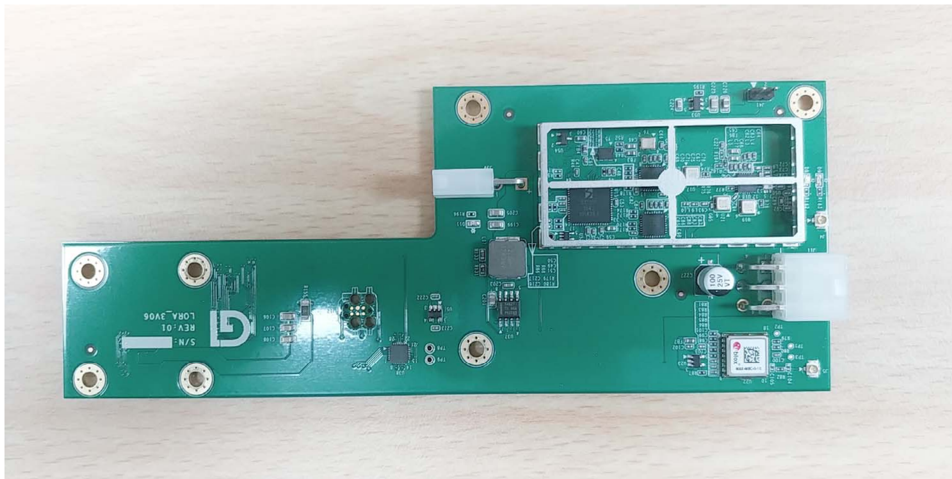
[Sub Board (Top)]
