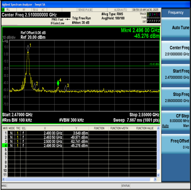
BLE_125K-Ant1-2480-PASS
