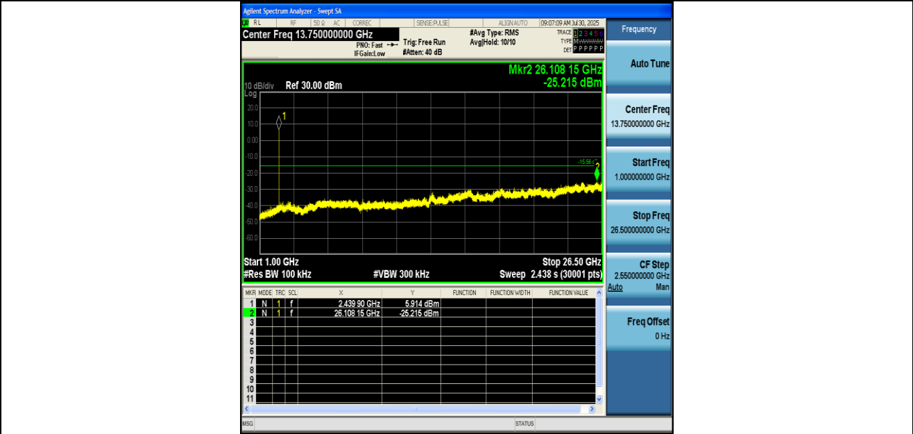
BLE_500K-Ant1-2440-1000~26500-PASS
