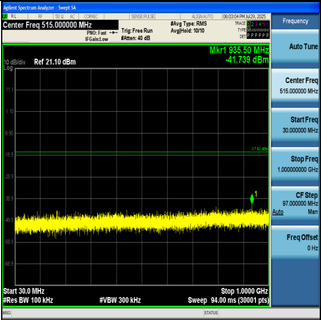
BLE_125K-Ant1-2402-30~1000-PASS
