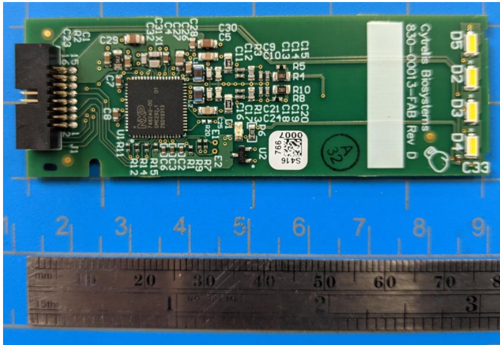
1 – Top-side
