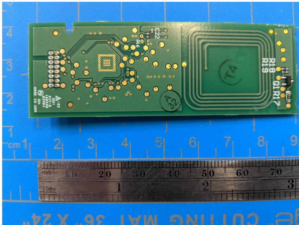
2 – Bottom side
