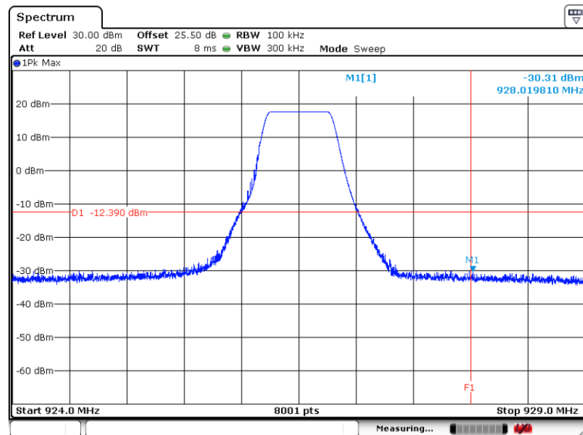
High Band Edge Plot on Channel 31
