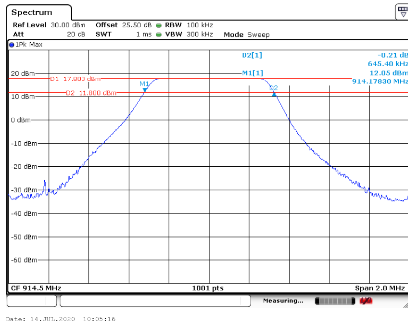
6 dB Bandwidth Plot on Channel 16
