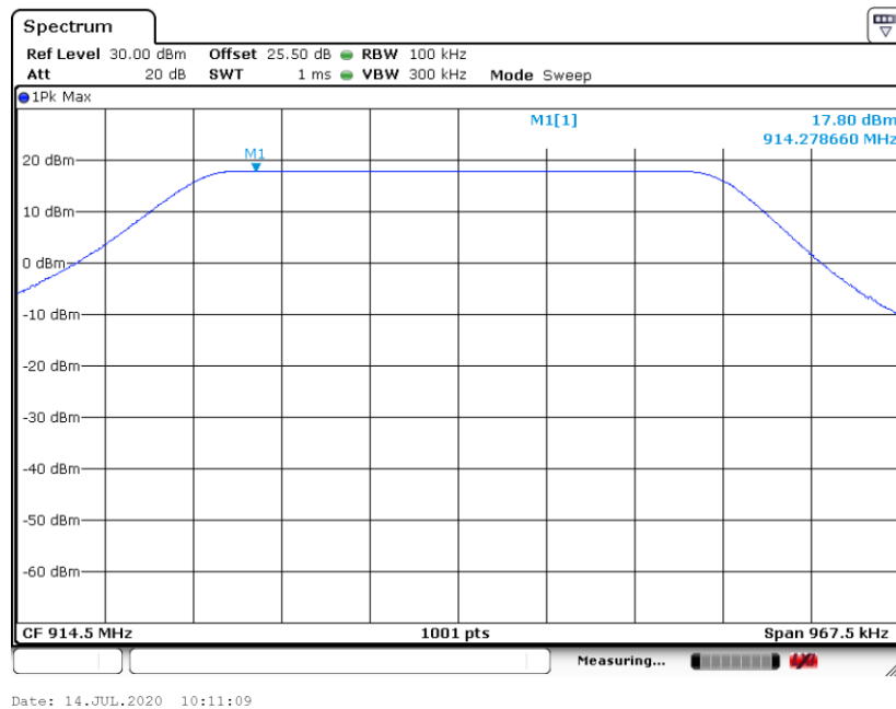
PSD 100kHz Plot on Channel 16
