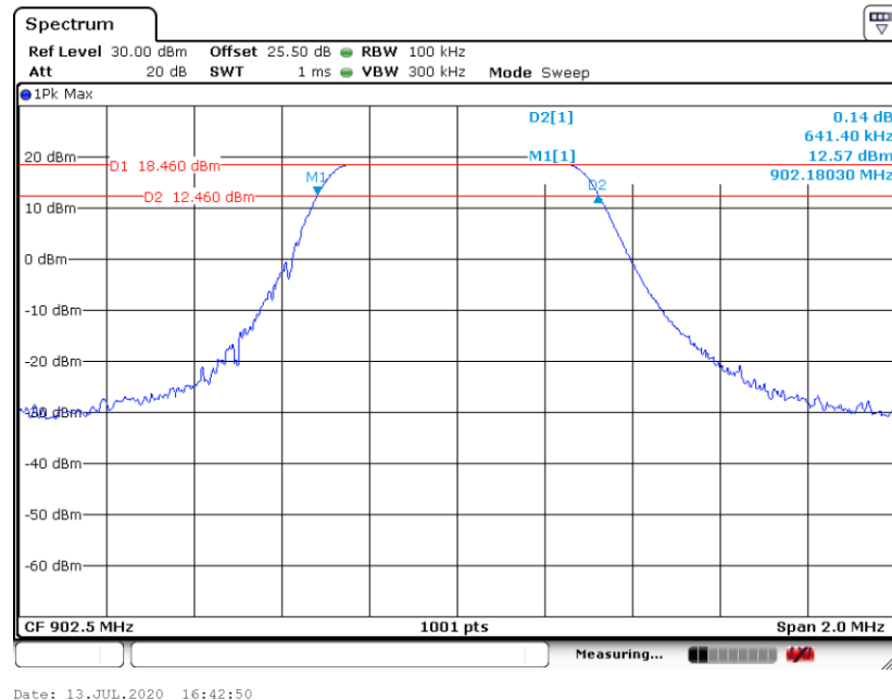
6 dB Bandwidth Plot on Channel 01
