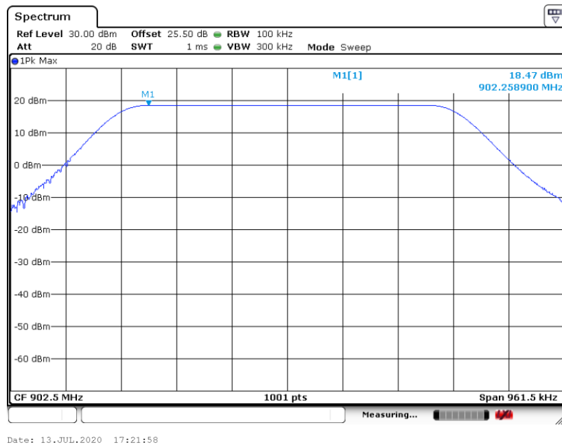
PSD 100kHz Plot on Channel 01
