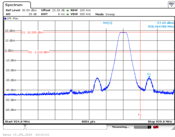
High Band Edge Plot on Channel 51
