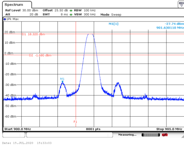
Low Band Edge Plot on Channel 01
