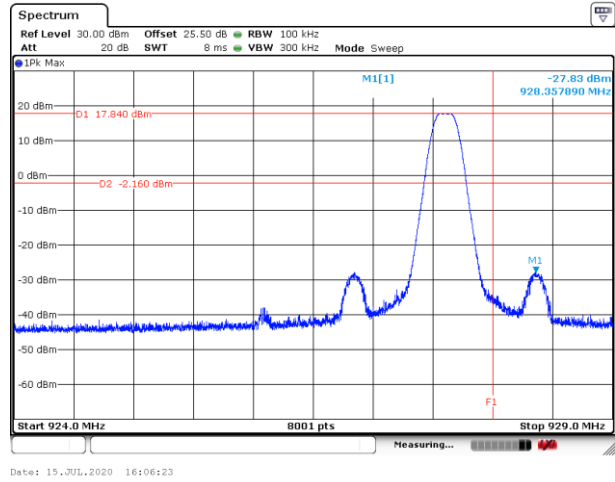
High Band Edge Plot on Channel 64
