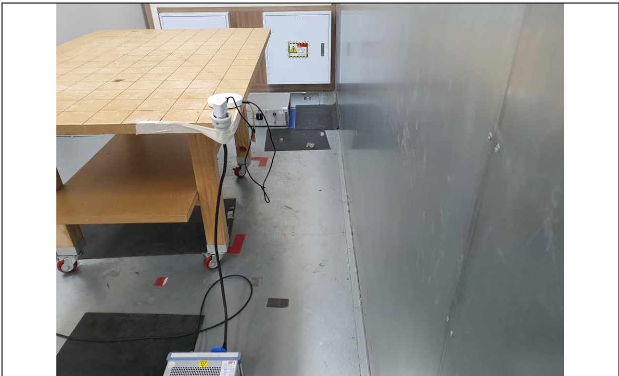
Conducted Emission_REAR
