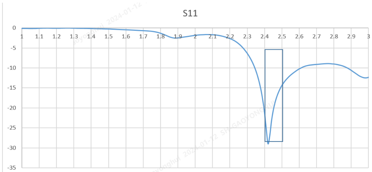
2.4G antenna S11
