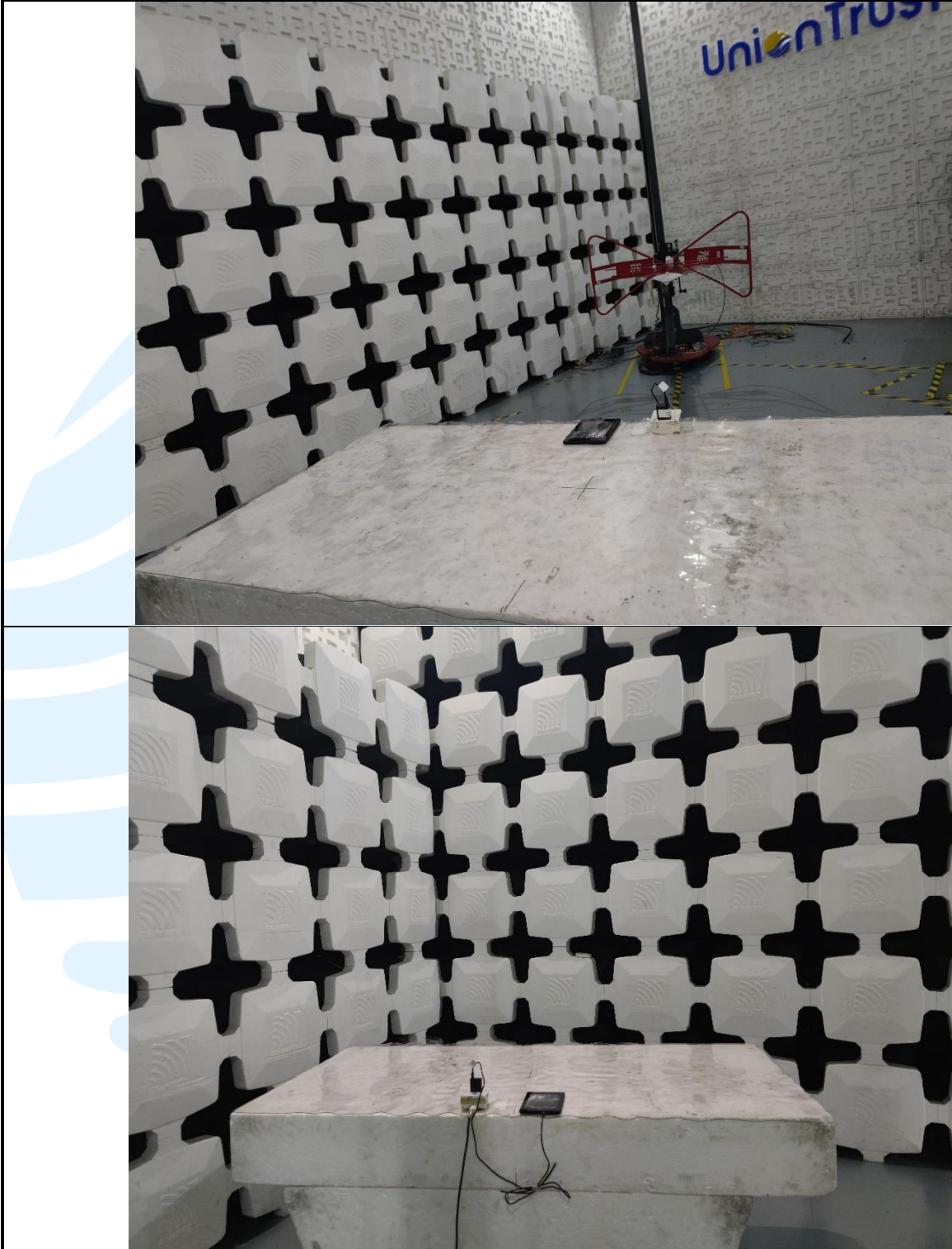
Radiated emission Test Setup (30 MHz~1 GHz)
