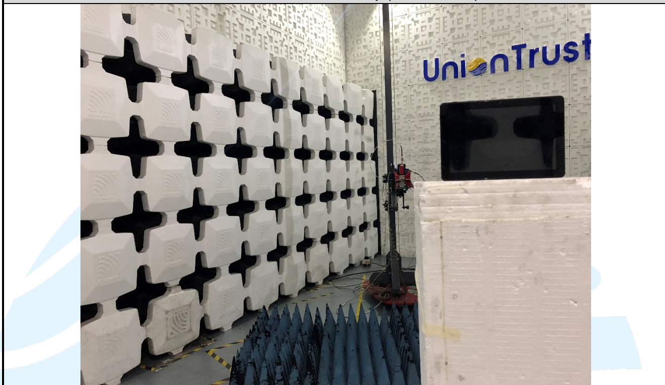
Radiated emission Test Setup (Above 1 GHz)
