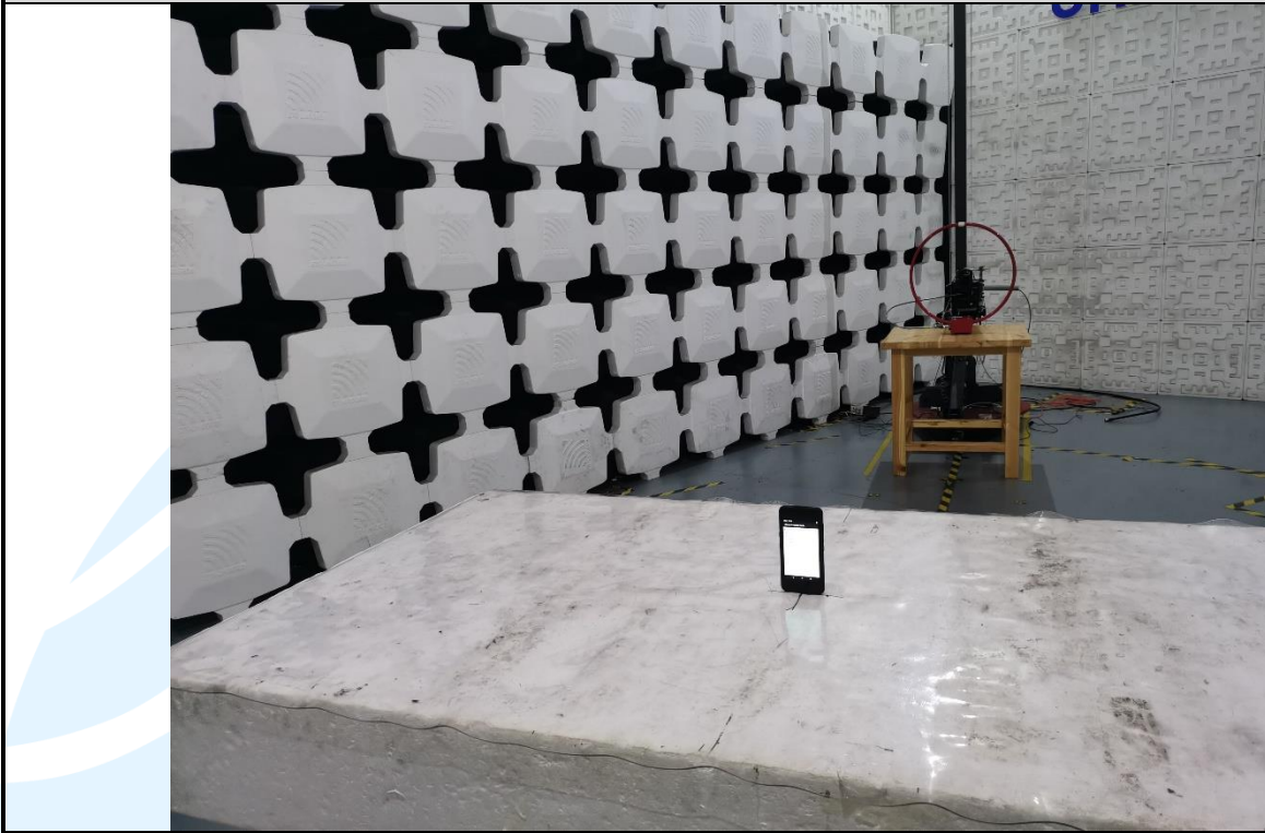
Radiated emission Test Setup (9kHz~30 MHz)
