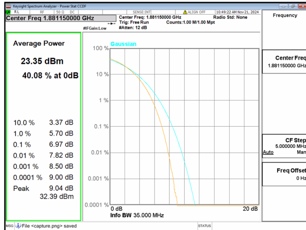
2C / 20+15MHz / Mid CH / 64QAM
