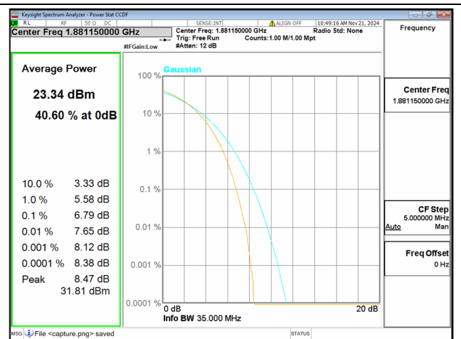
2C / 20+15MHz / Mid CH / 16QAM
