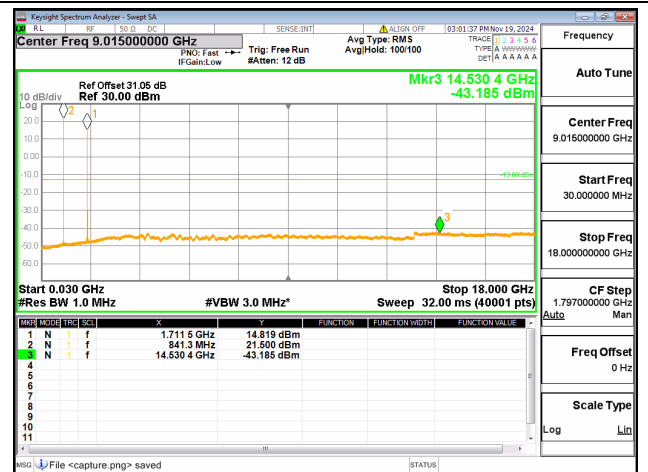
5A-66A / 10+20MHz / QPSK / Mid+Low CH / 1@49-1@0
