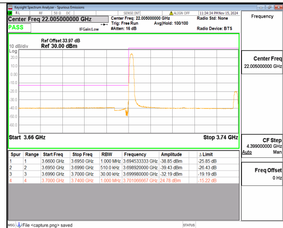
n78(3700-3800MHz) 40M DFT-s-OFDM 16QAM Edge_1RB_Left Low
