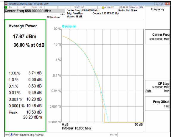
n71 10M CP-OFDM 256QAM Outer_Full Low
