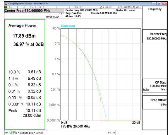
n71 20M CP-OFDM 256QAM Outer_Full Mid
