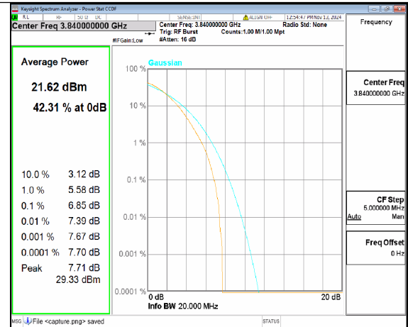
n77(3700-3980MHz) 20M DFT-s-OFDM 256QAM Outer_Full Mid
