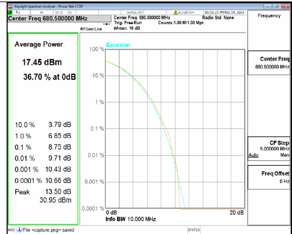
n71 10M CP-OFDM 256QAM Outer_Full Mid
