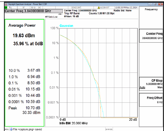
n77(3700-3980MHz) 20M CP-OFDM 256QAM Outer_Full Mid
