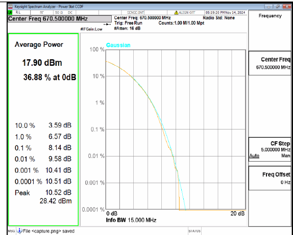
n71 15M CP-OFDM 256QAM Outer_Full Low
