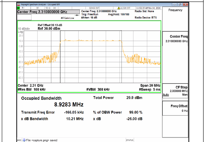
n30 10M DFT-s-OFDM 64QAM Outer_Full Mid
