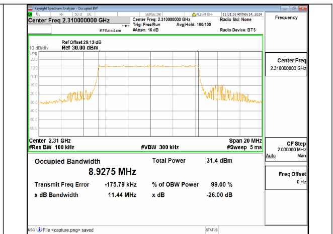
n30 10M DFT-s-OFDM QPSK Outer_Full Mid
