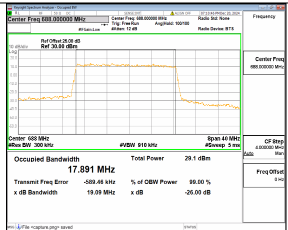
n71 20M DFT-s-OFDM 64QAM Outer_Full High
