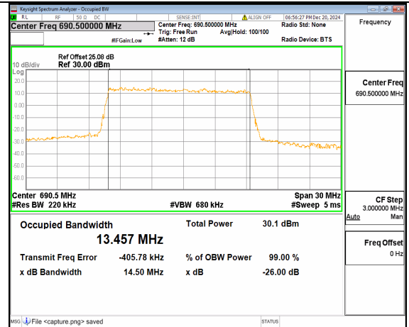
n71 15M DFT-s-OFDM QPSK Outer_Full High
