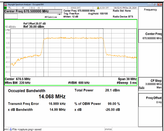
n71 15M CP-OFDM QPSK Outer_Full Low
