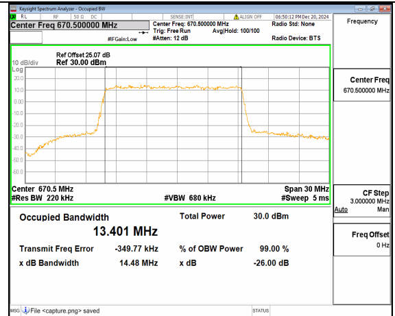
n71 15M DFT-s-OFDM QPSK Outer_Full Low
