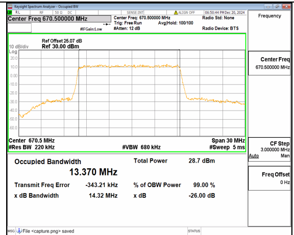
n71 15M DFT-s-OFDM 64QAM Outer_Full Low
