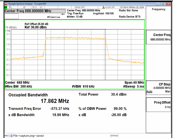
n71 20M DFT-s-OFDM QPSK Outer_Full High
