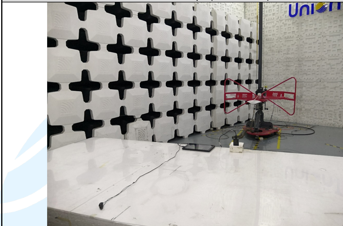
Radiated emission Test Setup-1 (30 MHz~1 GHz) - Mode 1
