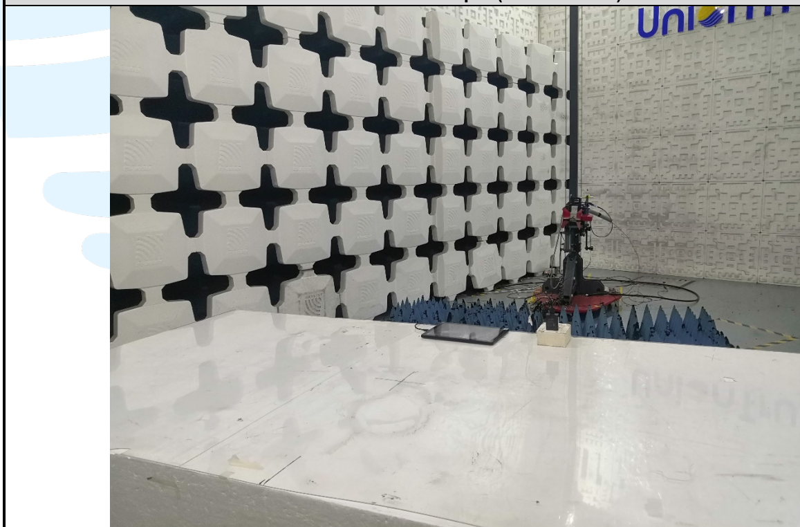
Radiated emission Test Setup-2 (Above 1 GHz) - Mode 2
