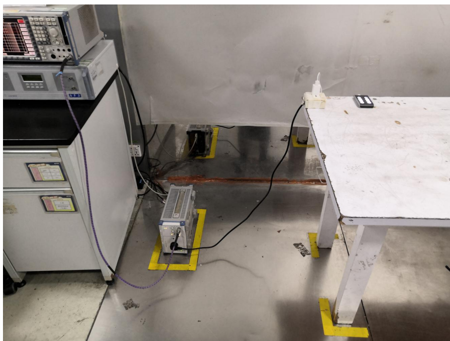
Conducted Emissions
