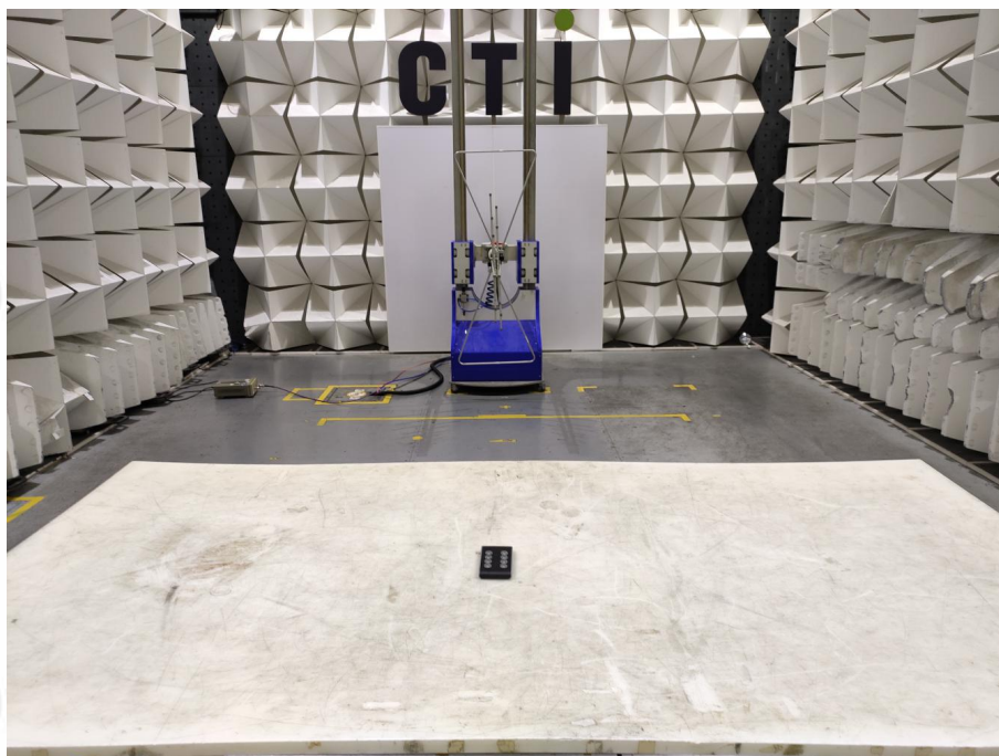
Radiated emission Test Setup-2 (Below 1GHz)
