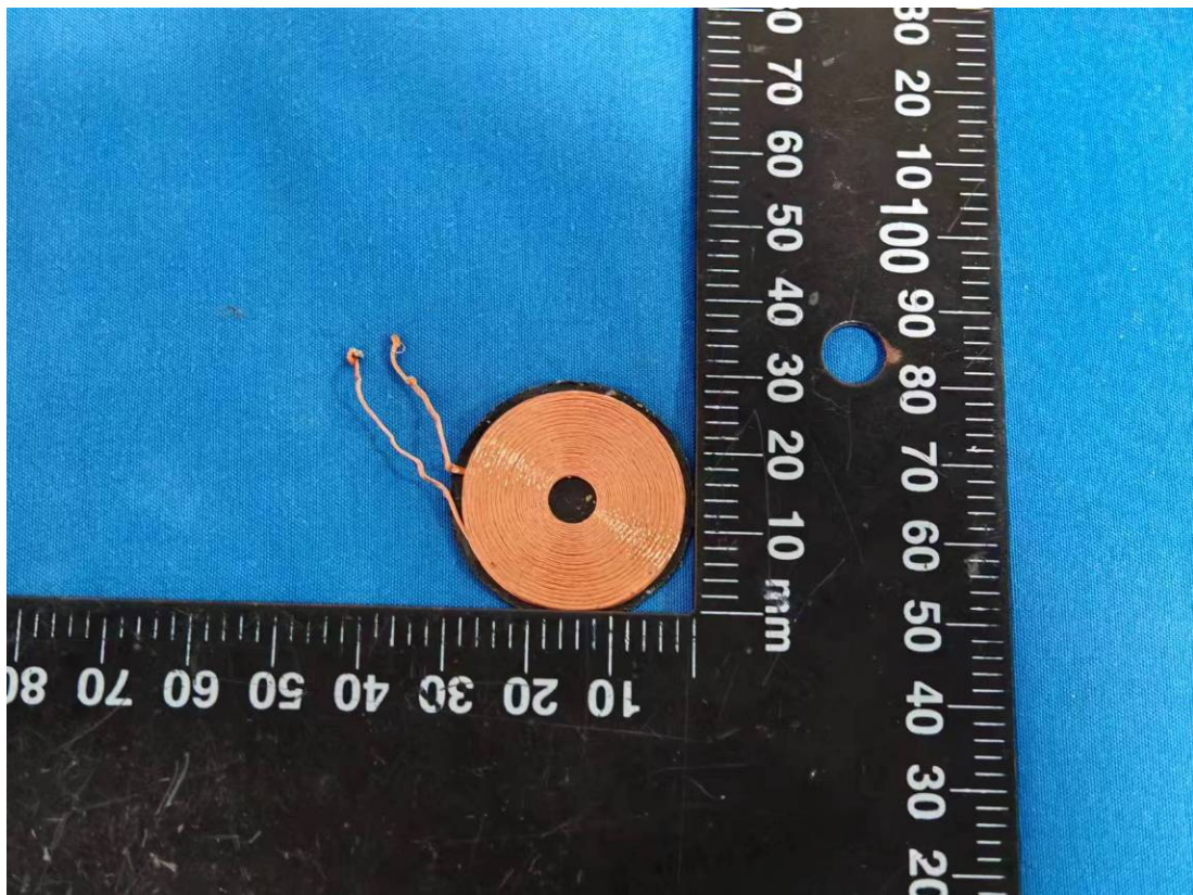
Wireless charger-Passive Coil
