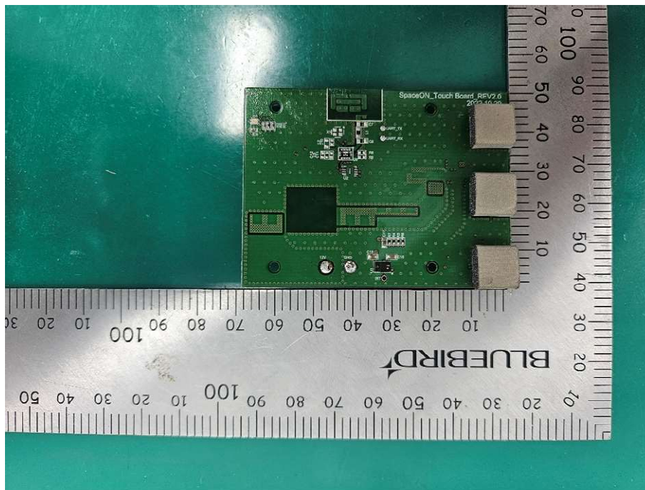
Touch Board - Front
