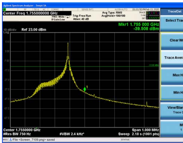
NB-IOT Band 4 QPSK 3.75KHz 1@0 CH-High
