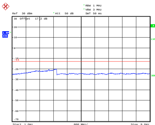
LTE Band 12 10MHz CH-Low 1GHz ~9GHz
