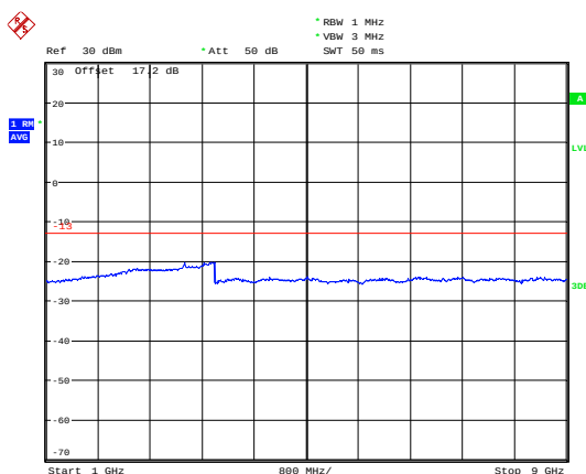
LTE Band 12 10MHz CH-High 1GHz ~9GHz
