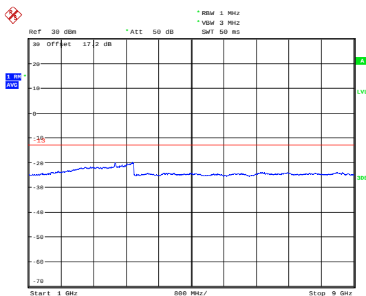
LTE Band 12 10MHz CH-Middle 1GHz ~9GHz
