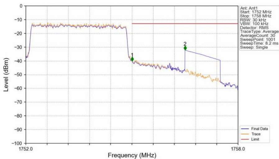
Band4_3MHz_16QAM_HCH_1753.5MHz_RB_15_0_NTNV
