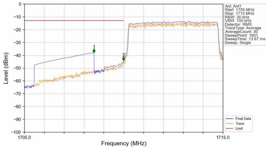
Band4_5MHz_QPSK_LCH_1712.5MHz_RB_25_0_NTNV
