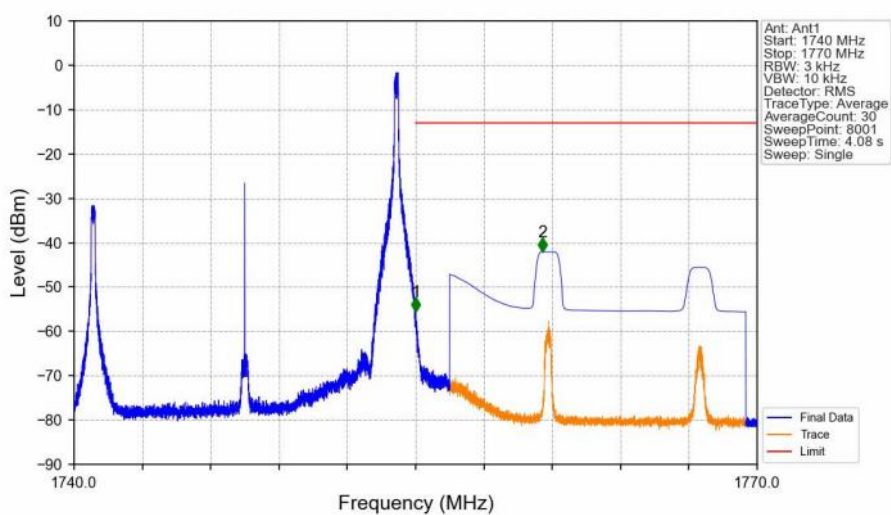
Band4_15MHz_16QAM_HCH_1747.5MHz_RB_1_74_NTNV
