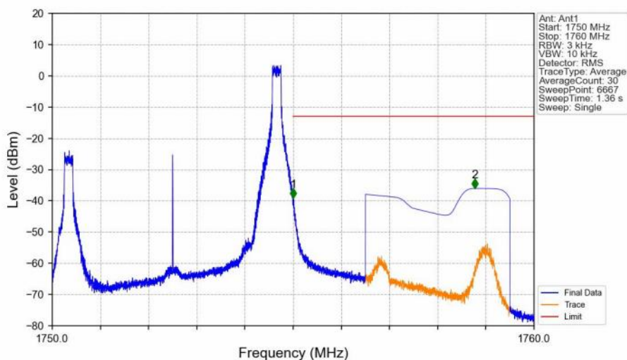
Band4_5MHz_16QAM_HCH_1752.5MHz_RB_1_24_NTNV
