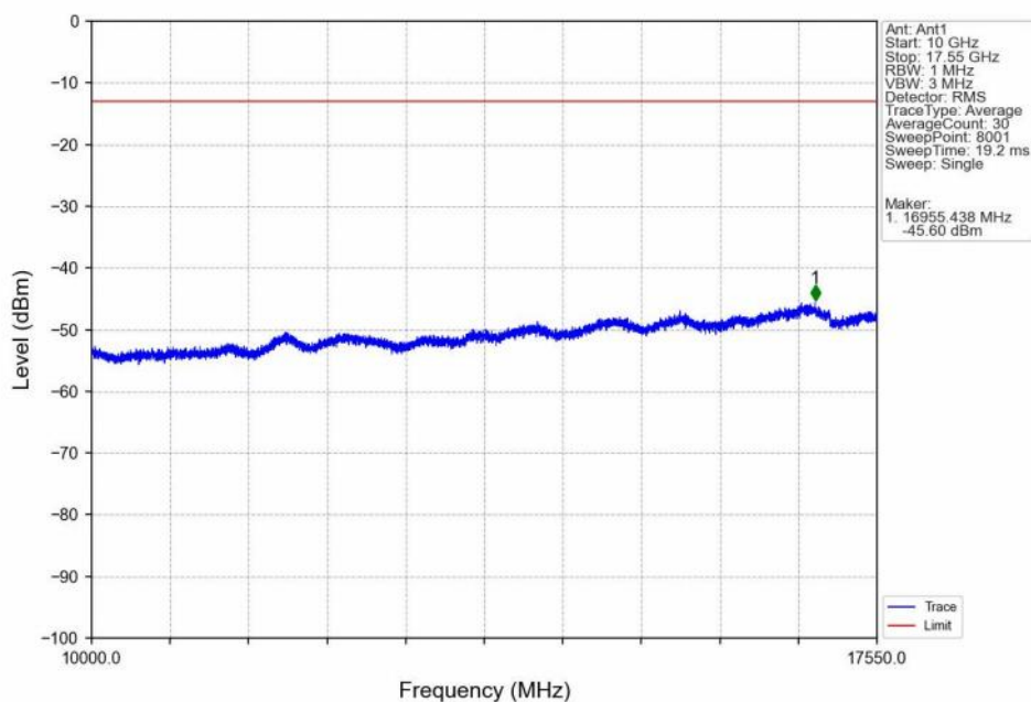
Band4_20MHz_16QAM_HCH_1745MHz_RB_1_99_NTNV
