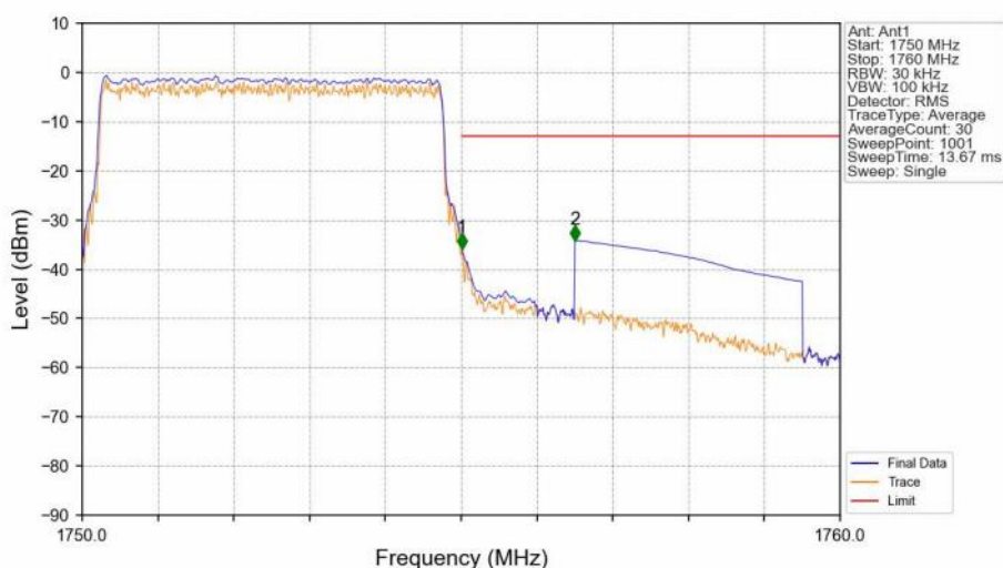
Band4_5MHz_16QAM_HCH_1752.5MHz_RB_25_0_NTNV
