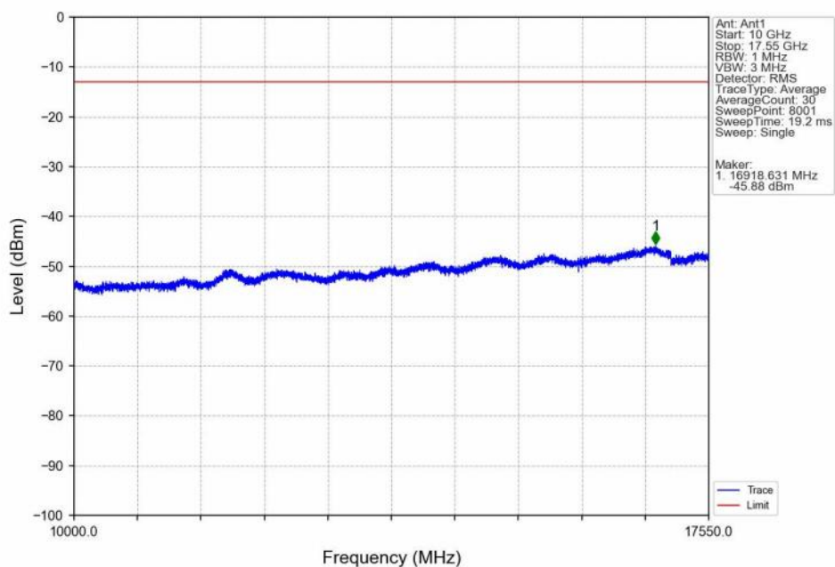
Band4_15MHz_16QAM_HCH_1747.5MHz_RB_1_74_NTNV
