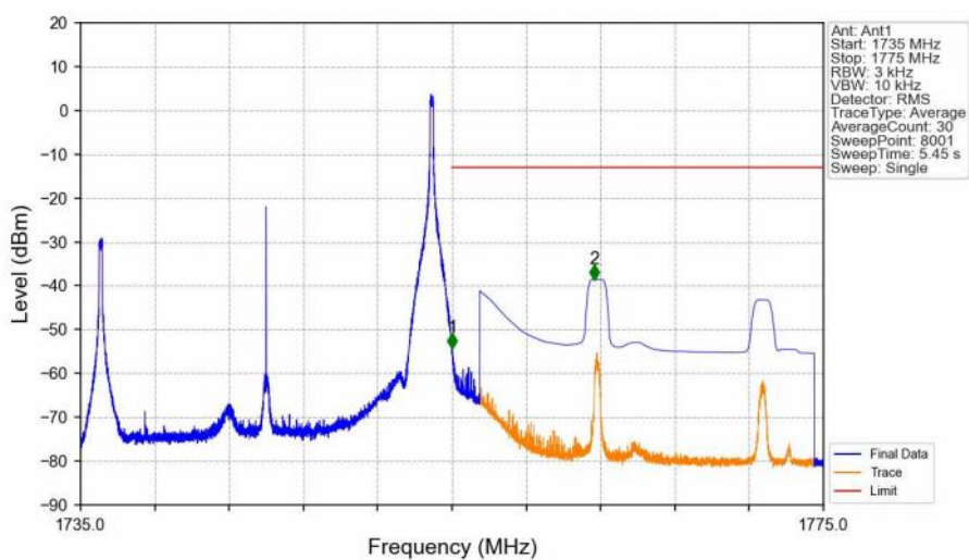
Band4_20MHz_16QAM_HCH_1745MHz_RB_1_99_NTNV
