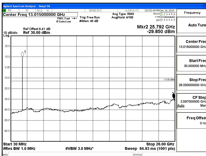
(Channel Bandwidth: 5 MHz)_LCH_QPSK_1RB#12
