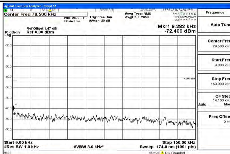
Band4-3MHz-16QAM-20385-1RB#0-Range2:0.15~30MHz
