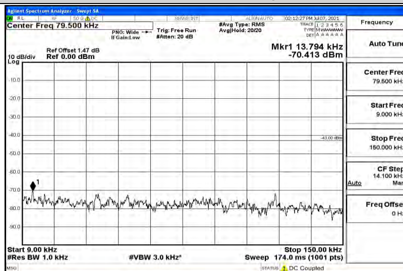
Band2-1.4MHz-16QAM-19193-1RB#0-Range2:0.15~30MHz
