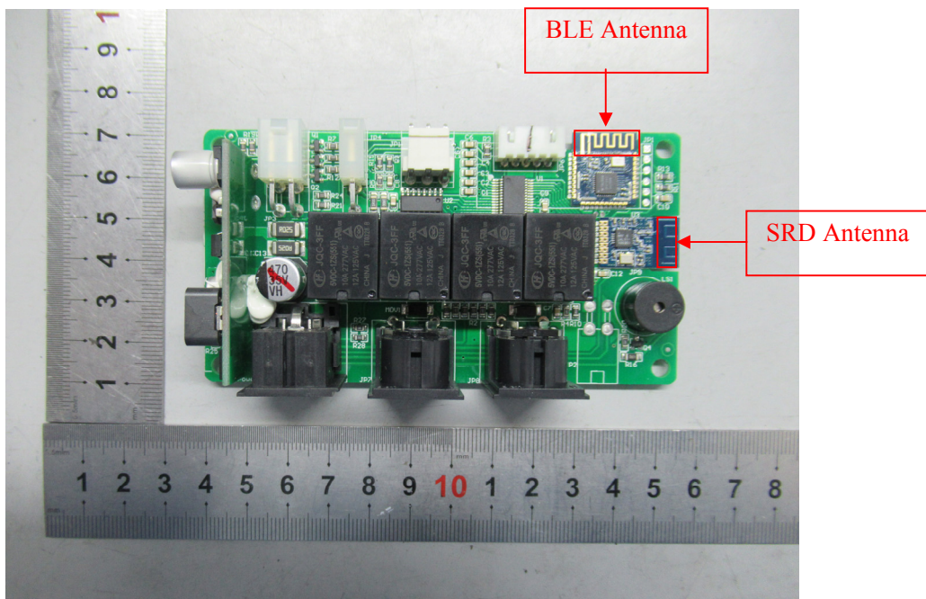
EUT – PCB-1 Top Shielding off View
