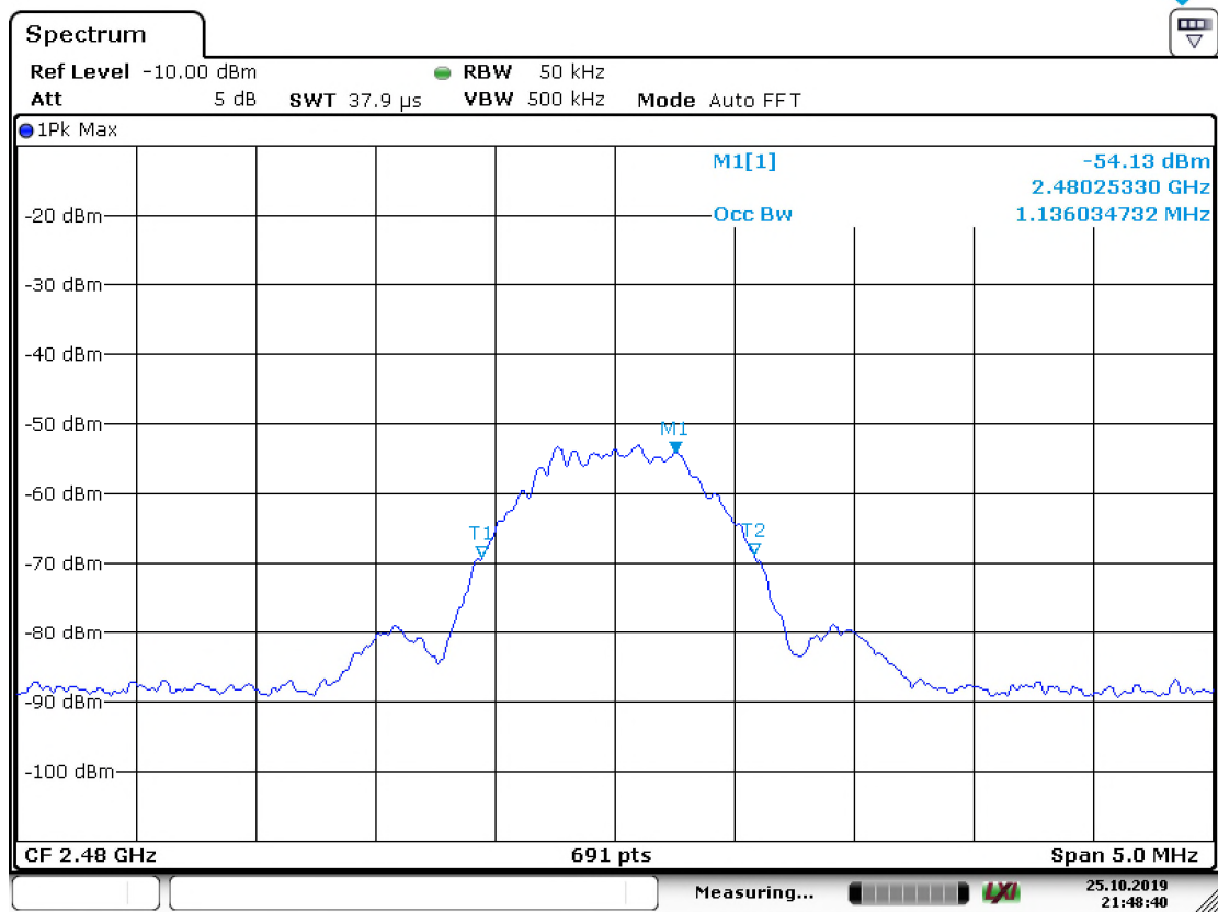
Graphs 8: Results- OBW Results – Top
