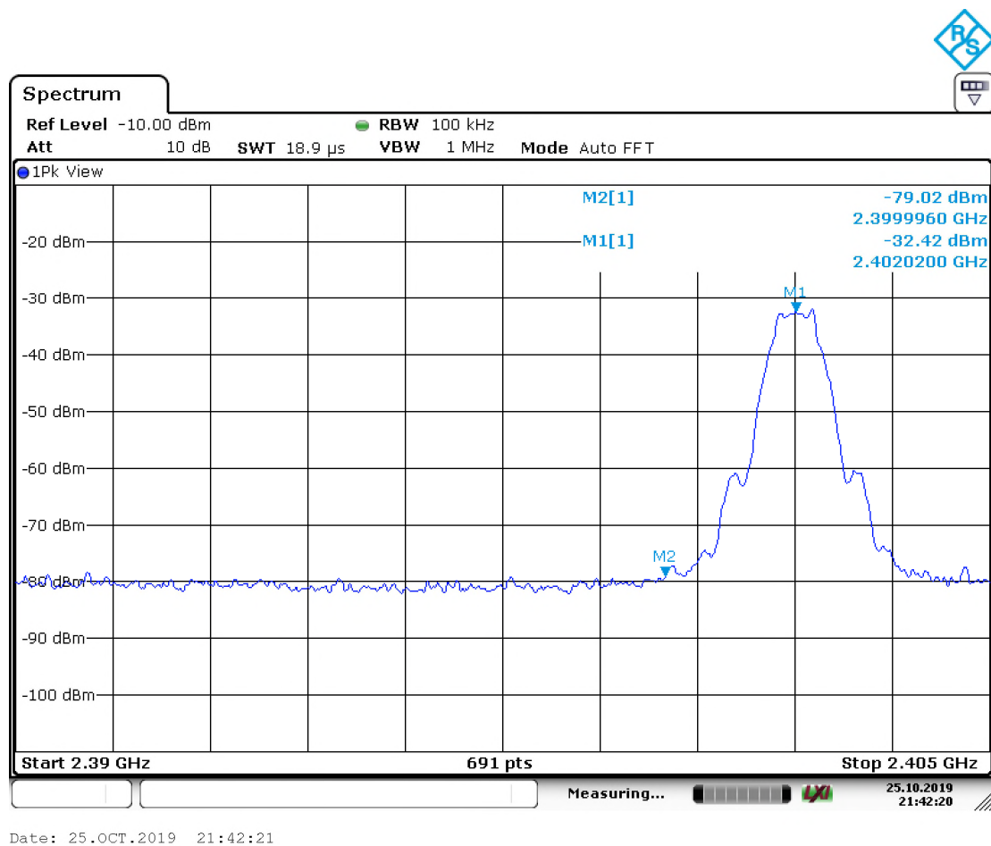
Graph 9: Results – 20 dBc Low channel
