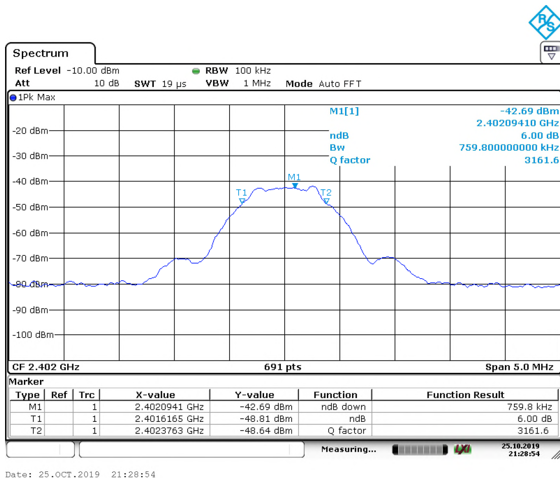
Graphs 5: 6dB Results – Low
