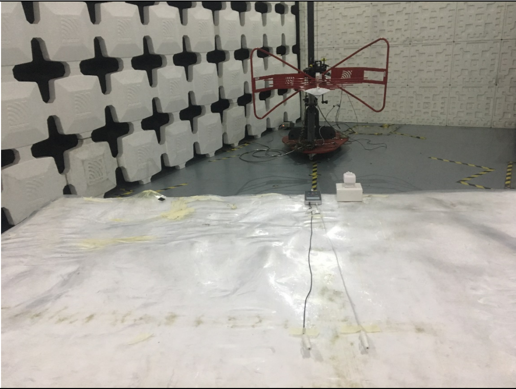
Radiated emission Test Setup-2 (30 MHz~1 GHz) - Mode 1
