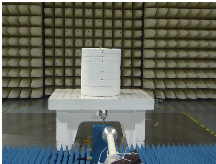
Figure 3: Test Setup for Radiated Emissions 18GHz to 26 GHz
