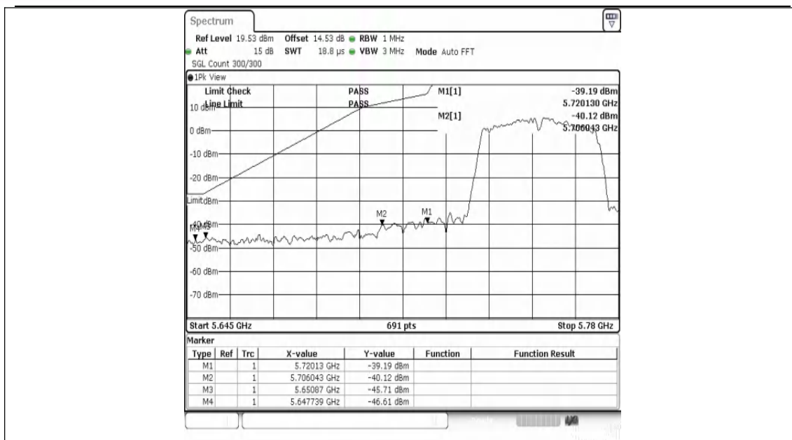
11AC40SISO-Ant1-5755-PASS
