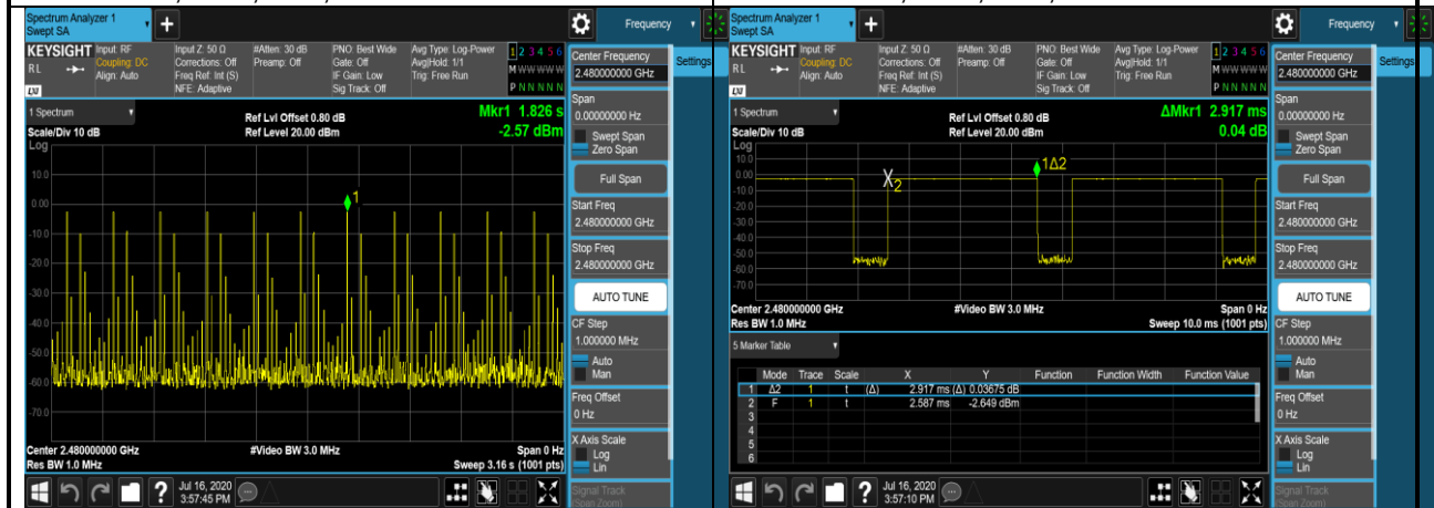
GFSK,2480,DH5,Transmission Number
