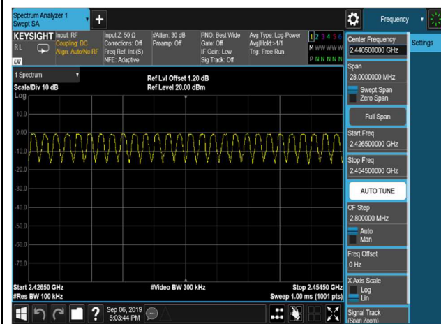
GFSK,Hopping,DH5,2426.5~2454.5MHz
