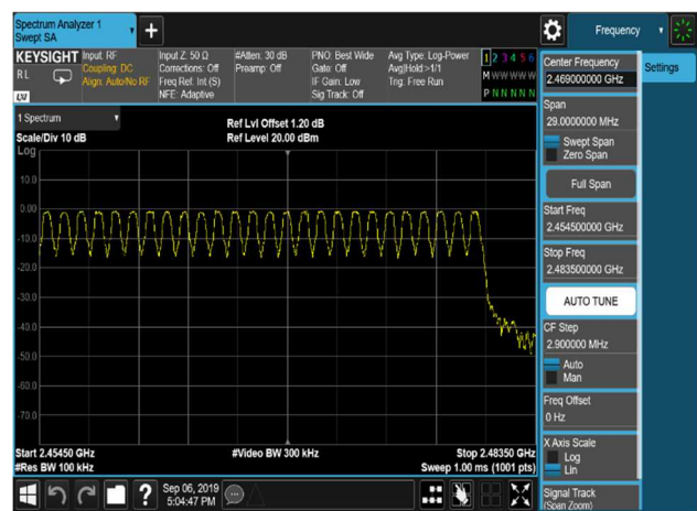
GFSK,Hopping,DH5,2454.5~2483.5MHz
