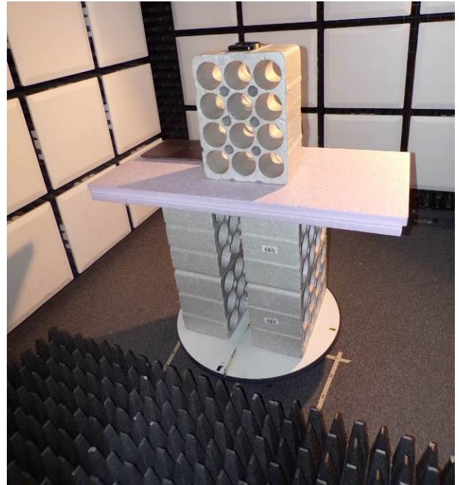
FAC setup (1GHz-25GHz / 3m)
