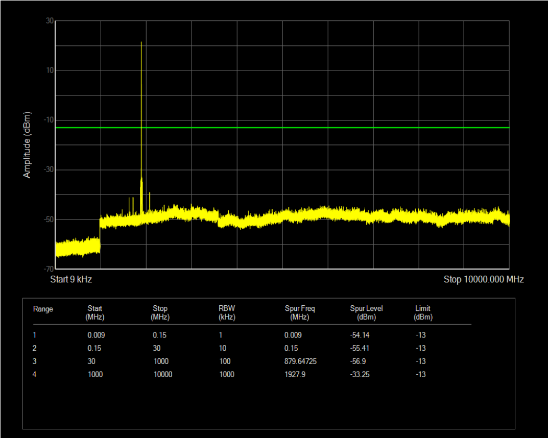
Band25 QAM16 BW=3MHz Channel=26675 RB Size=1 Position=#0 NB Index=0
