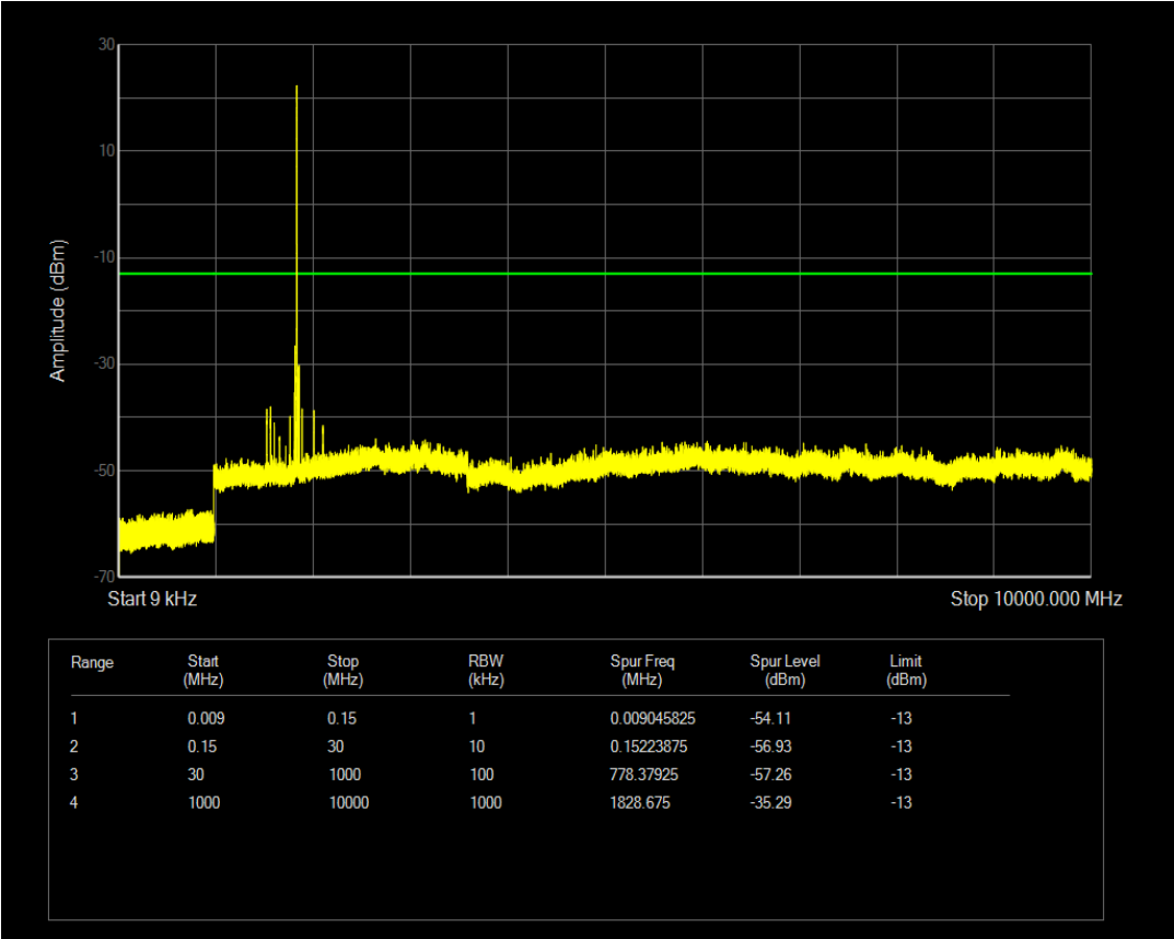
Band25 QAM16 BW=5MHz Channel=26065 RB Size=1 Position=#0 NB Index=0
