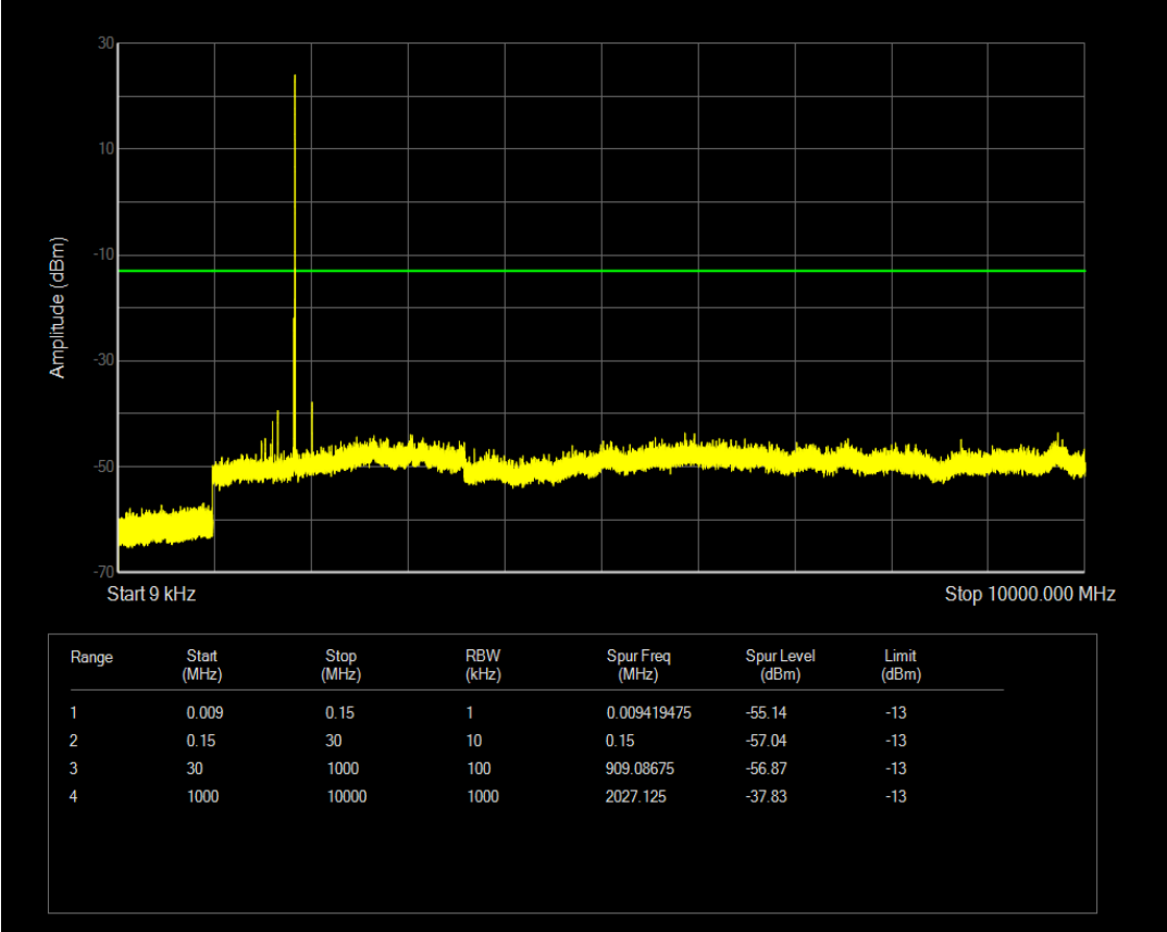
Band25 QAM16 BW=5MHz Channel=26065 RB Size=6 Position=#0 NB Index=0
