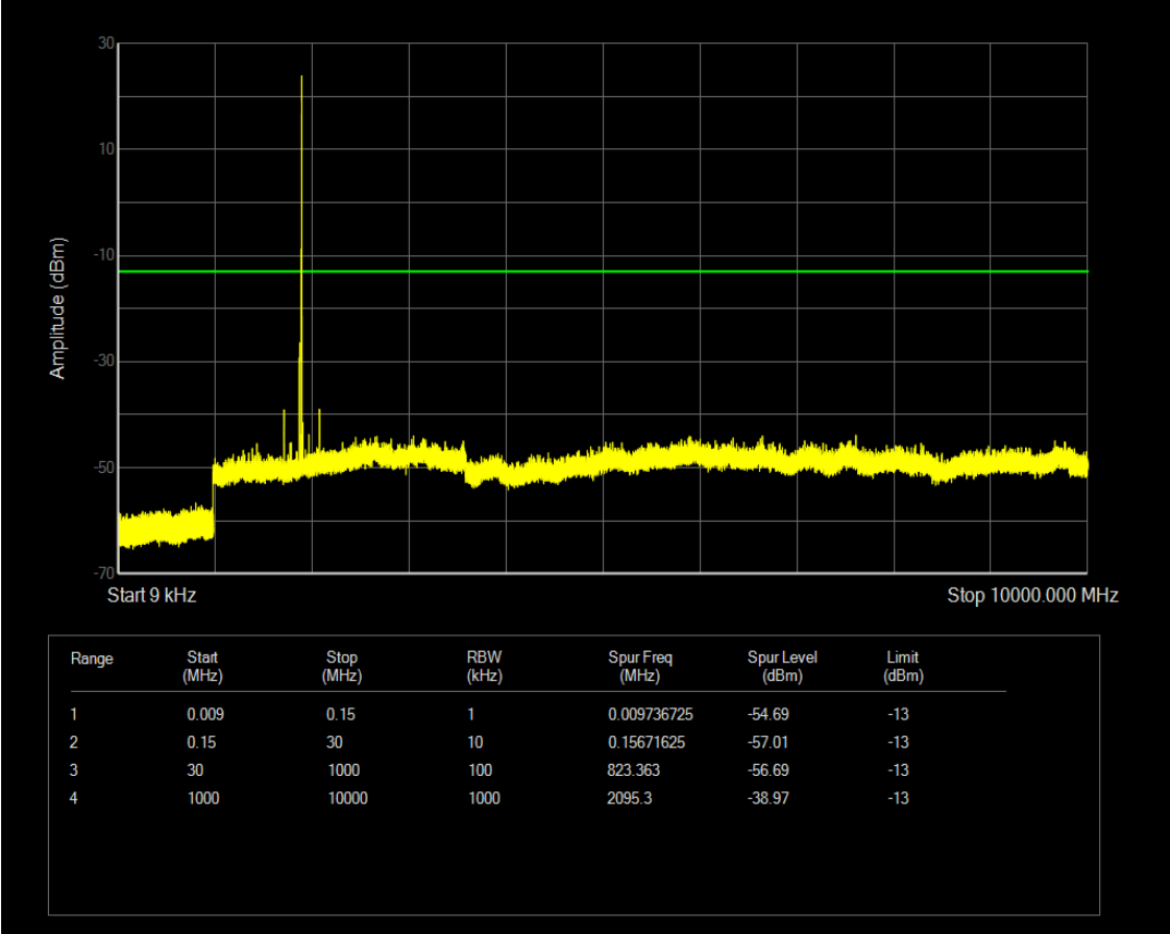
Band25 QAM16 BW=3MHz Channel=26675 RB Size=6 Position=#0 NB Index=0
