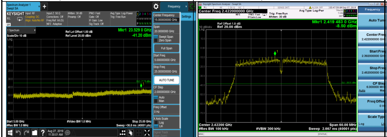
802.11n(HT40),2422MHz,Ant0,Plot 2,Band Edge
