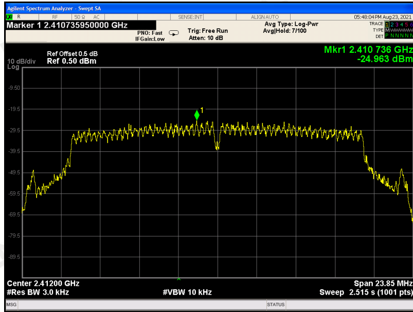
CH1: 2412MHz
